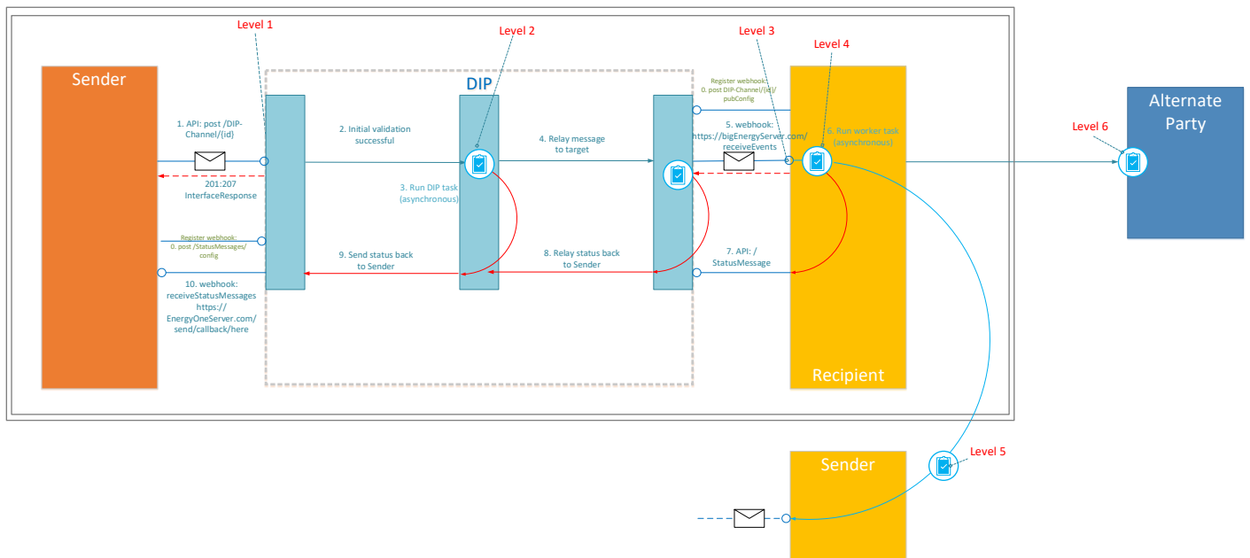
Figure 3 - Message Channel Pattern and validation levels
