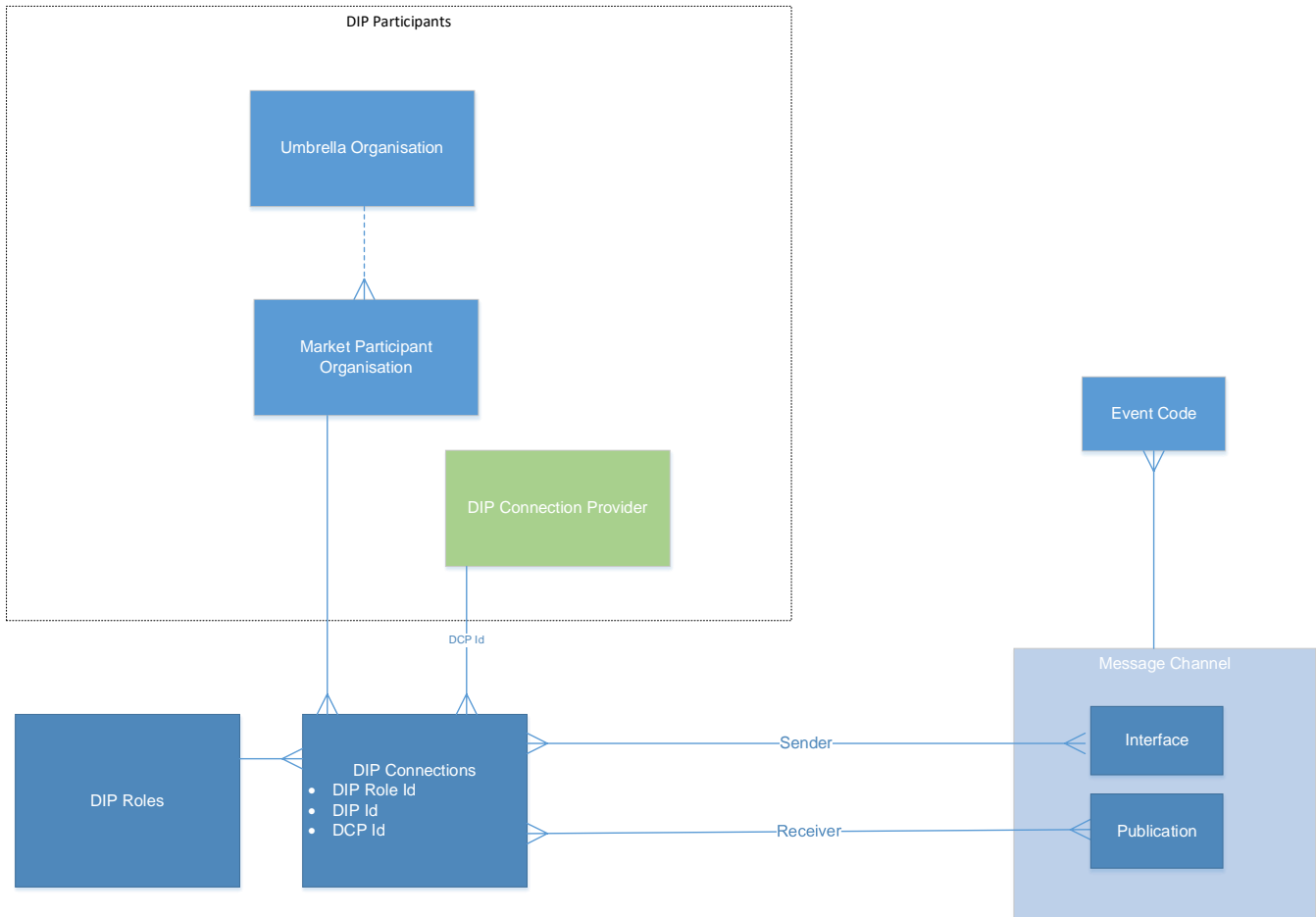
Figure 2 - DIP Workflows logical view
