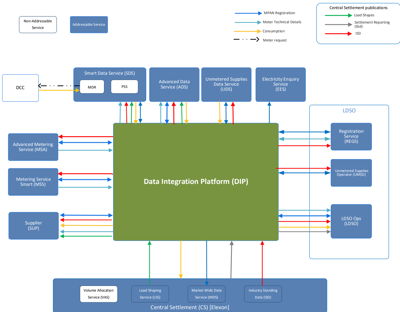
Figure 1 MHHS TOM Workflows
