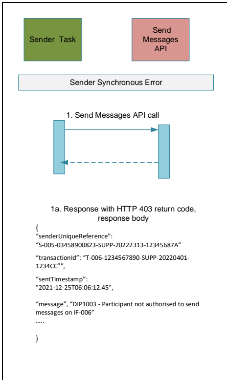
Figure 6 – Level 1 DIP Synchronous Error
