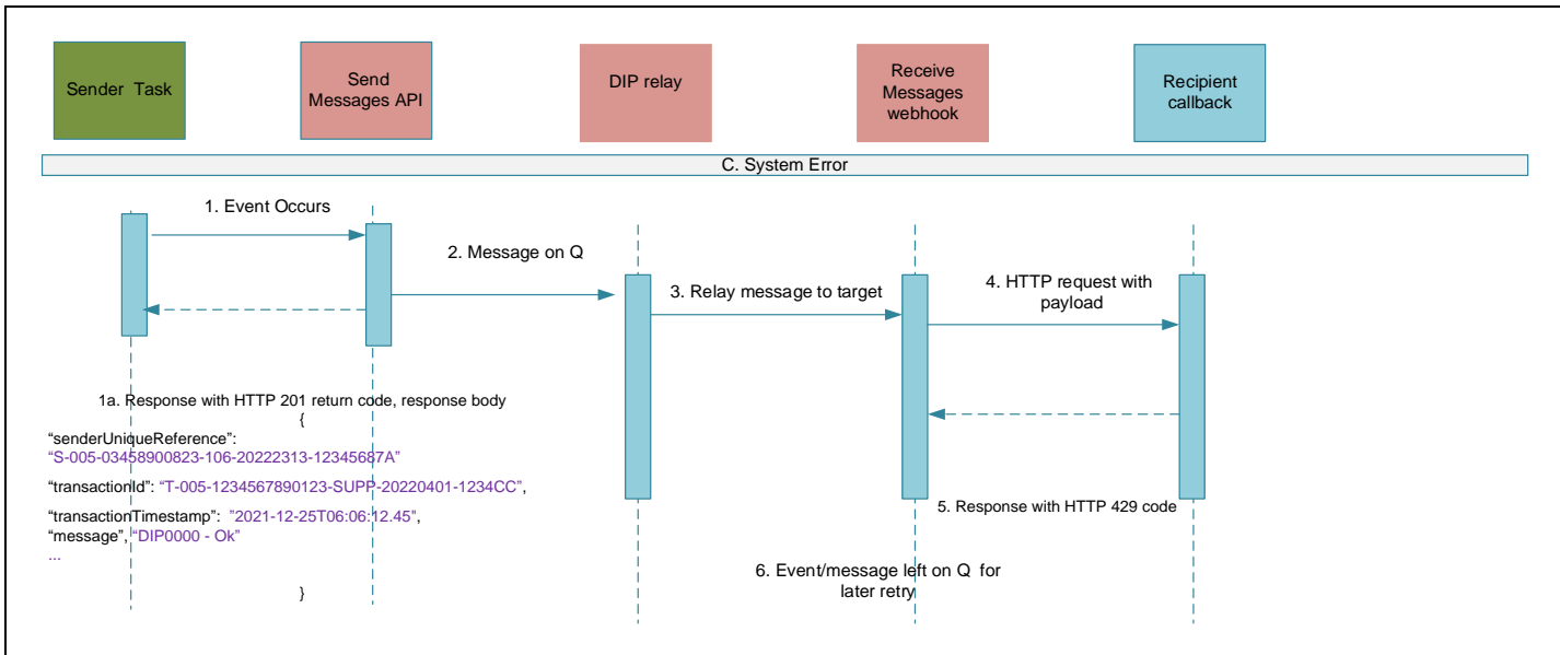
Figure 8 – Level 3 - Recipient Synchronous Error (retry)
