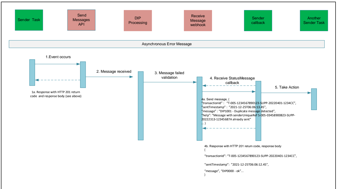
Figure 7 Level 2- DIP Asynchronous Error
