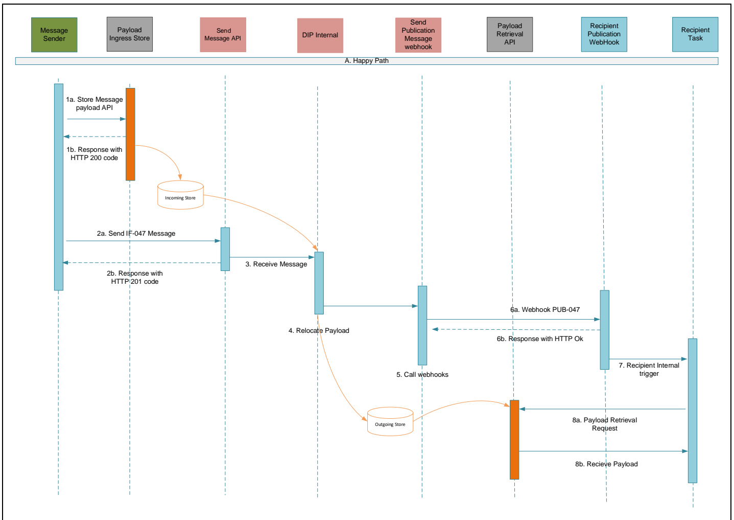
Figure 11 - Message Pattern 'B' Orchestration
