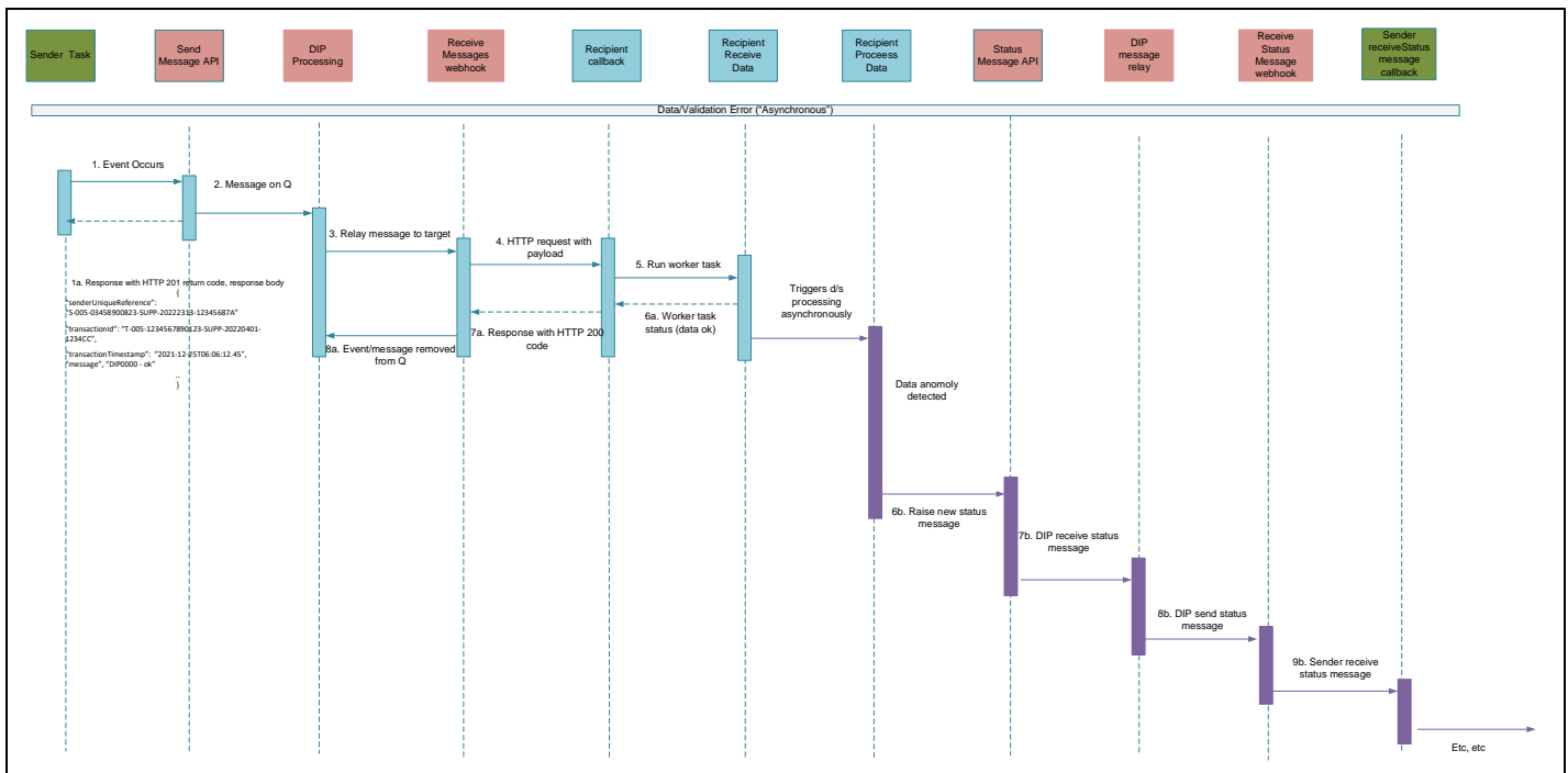
Figure 10 - Recipient Data Error - Asynchronous reporting
