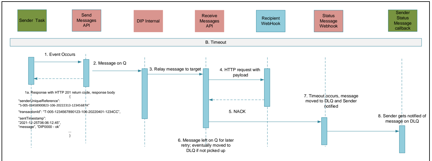
Figure 12 – Recipient Timeout
