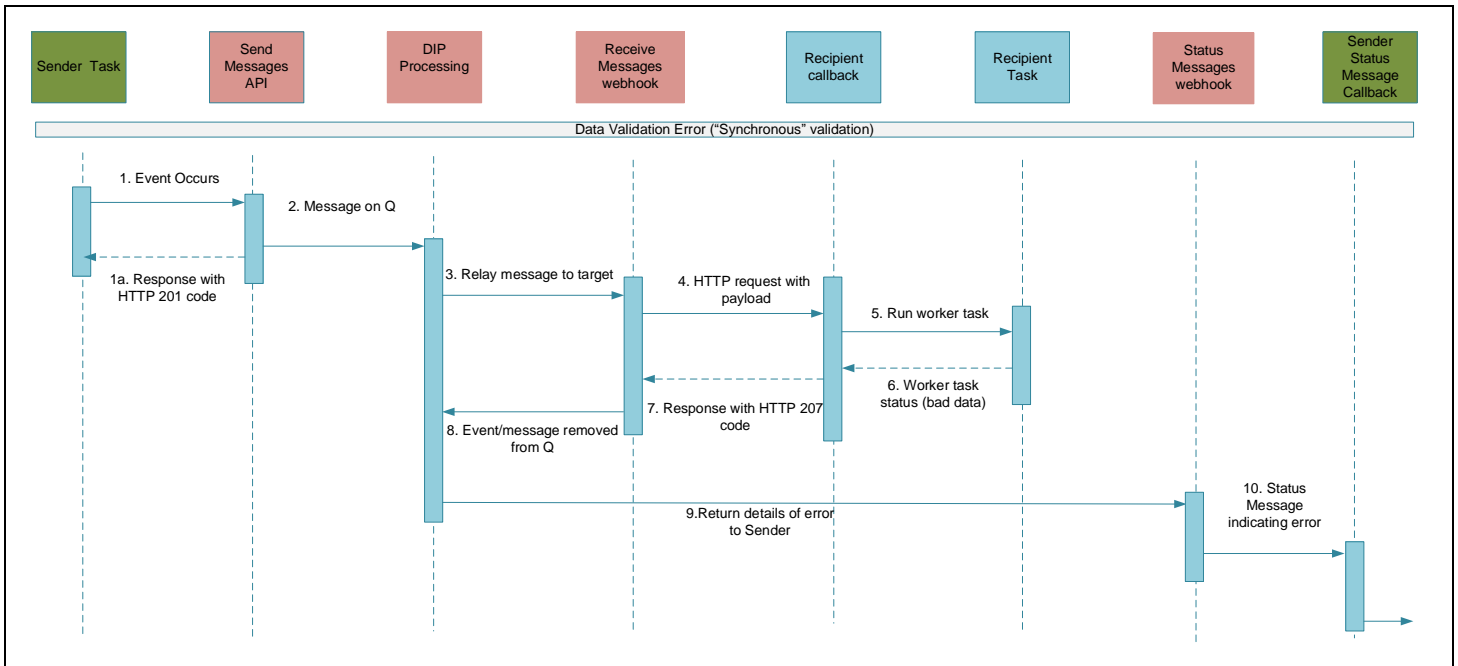
Figure 9 - Recipient synchronous Error (no-retry)
